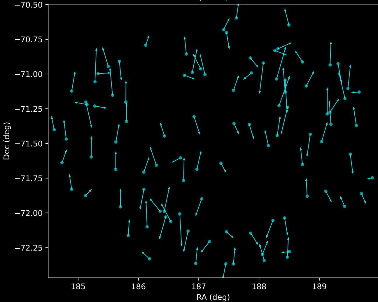
APOGEE DR17 Noise Stream Proper Motion Vectors (n=96)
