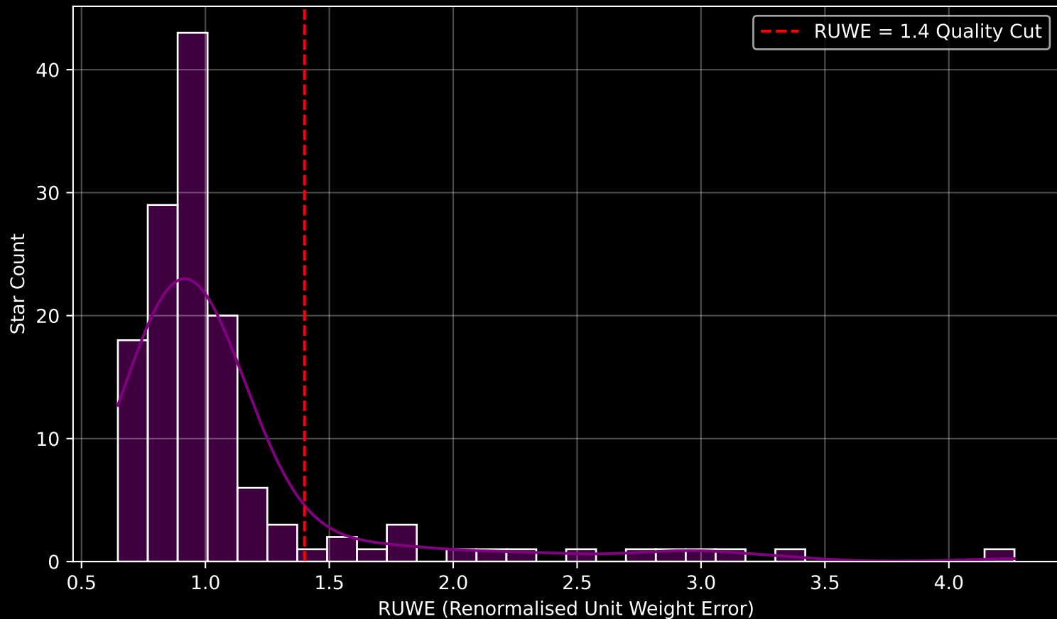
GAPOGEE DR17 Field [282-31-O_TESS] RUWE Distribution (n= 136)
