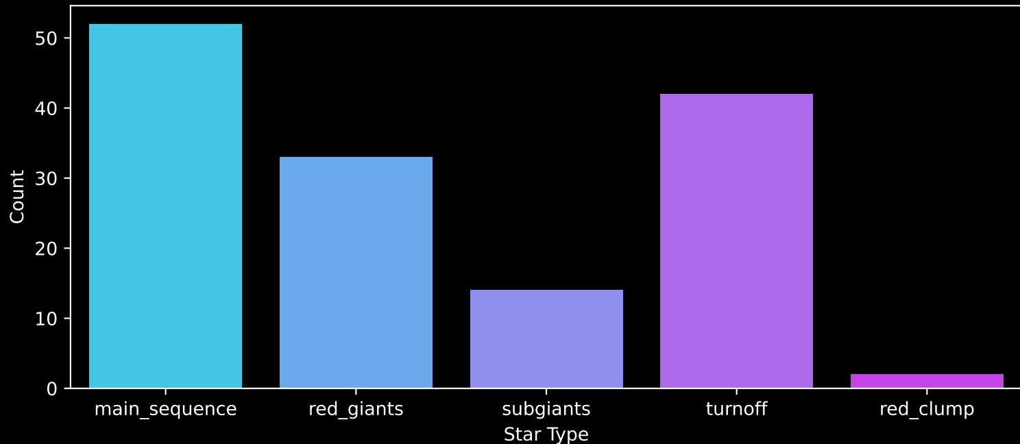
APOGEE DR17 Field: [282-31-O_TESS] Count plot of Star Type
